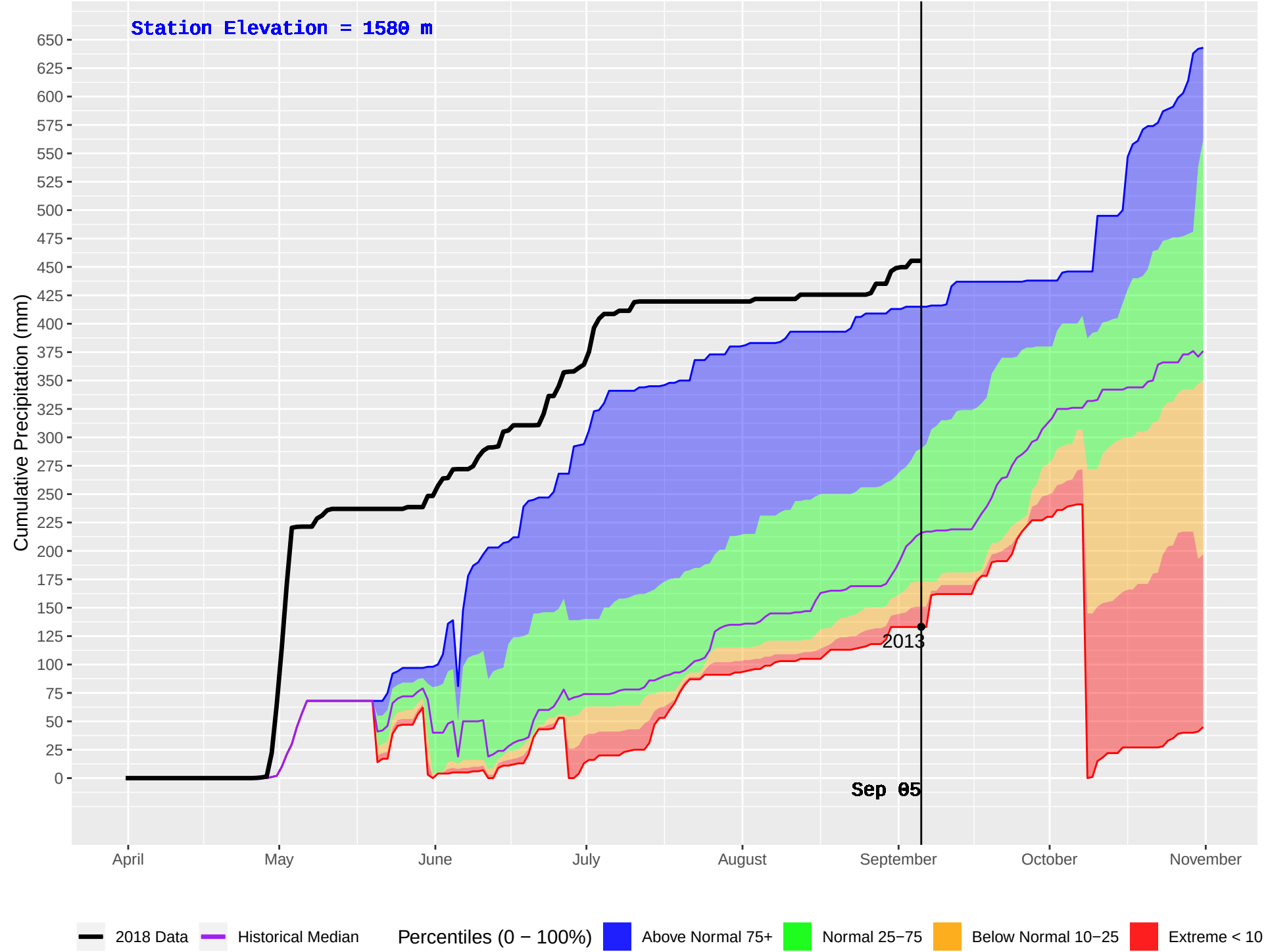
RORY CREEK (1092) : Historical (2010–2016) and Current (2018) Daily Cumulative Precipitation
