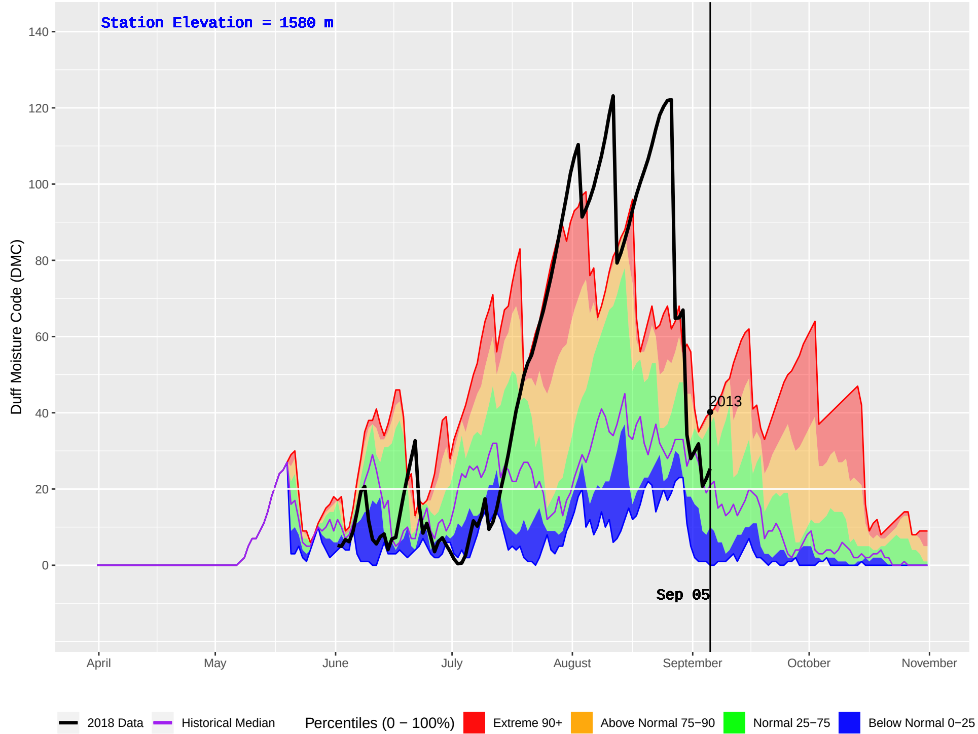
RORY CREEK (1092) : Historical (2010–2016) and Current (2018) Daily Duff Moisture Code (DMC)
