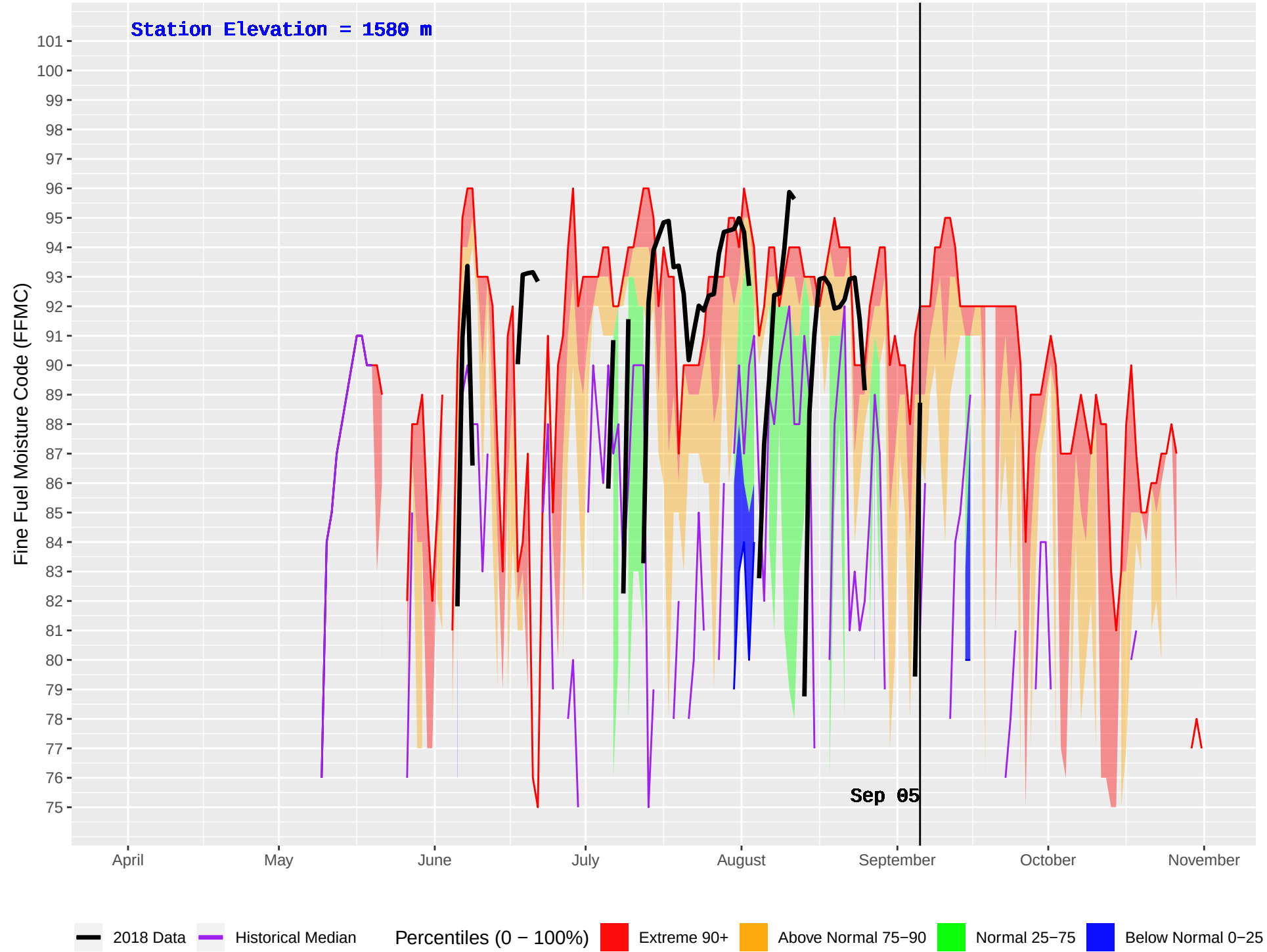
RORY CREEK (1092) : Historical (2010–2016) and Current (2018) Daily Fine Fuel Moisture Code (FFMC)
