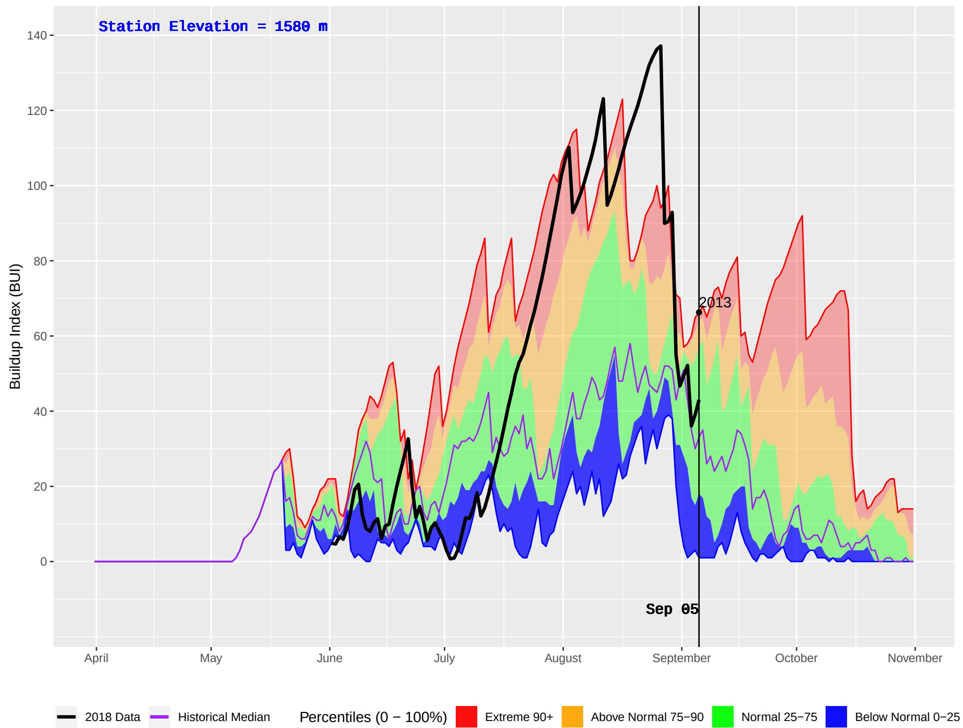
RORY CREEK (1092) : Historical (2010–2016) and Current (2018) Daily Buildup Index (BUI)
