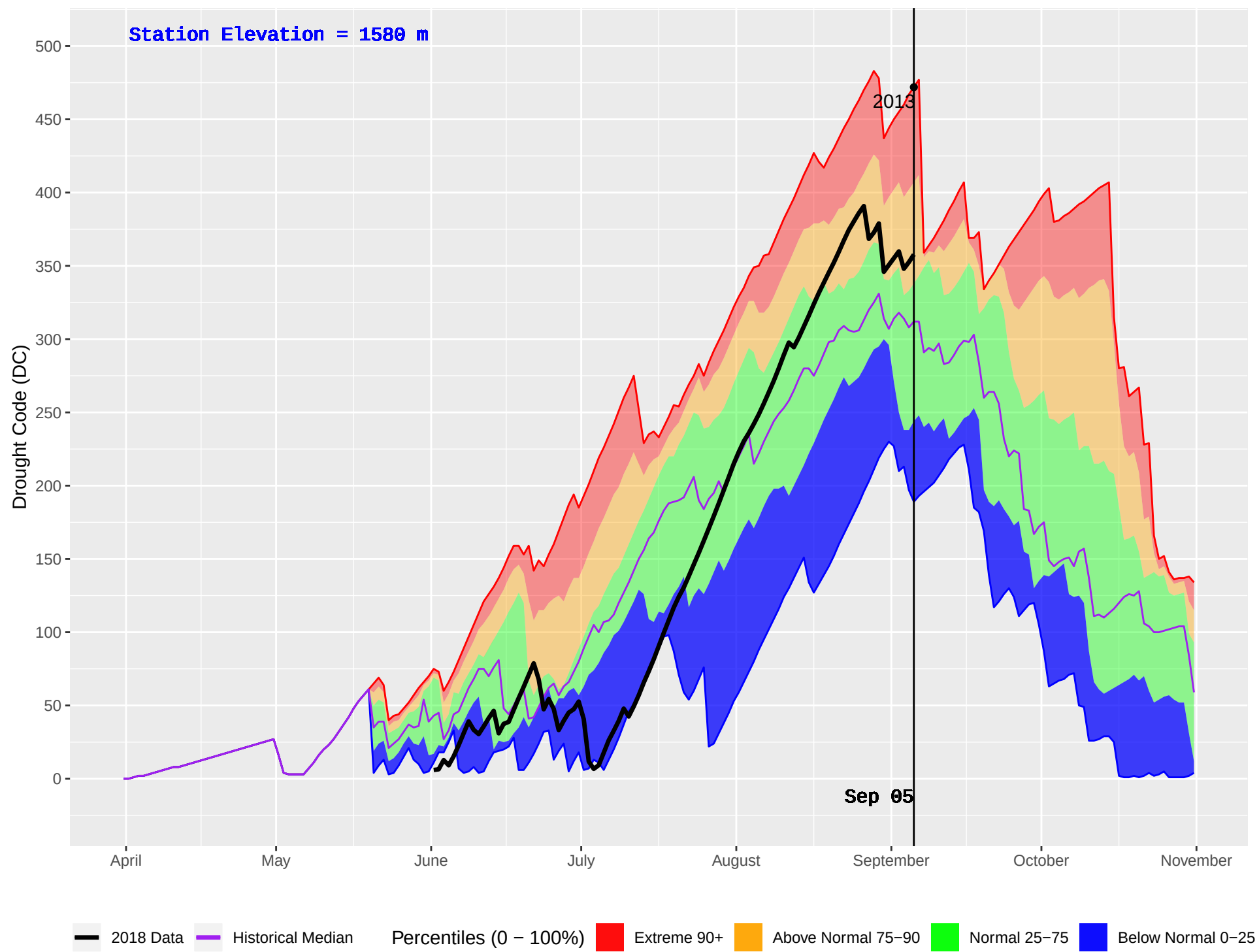
RORY CREEK (1092) : Historical (2010–2016) and Current (2018) Daily Drought Code (DC)
