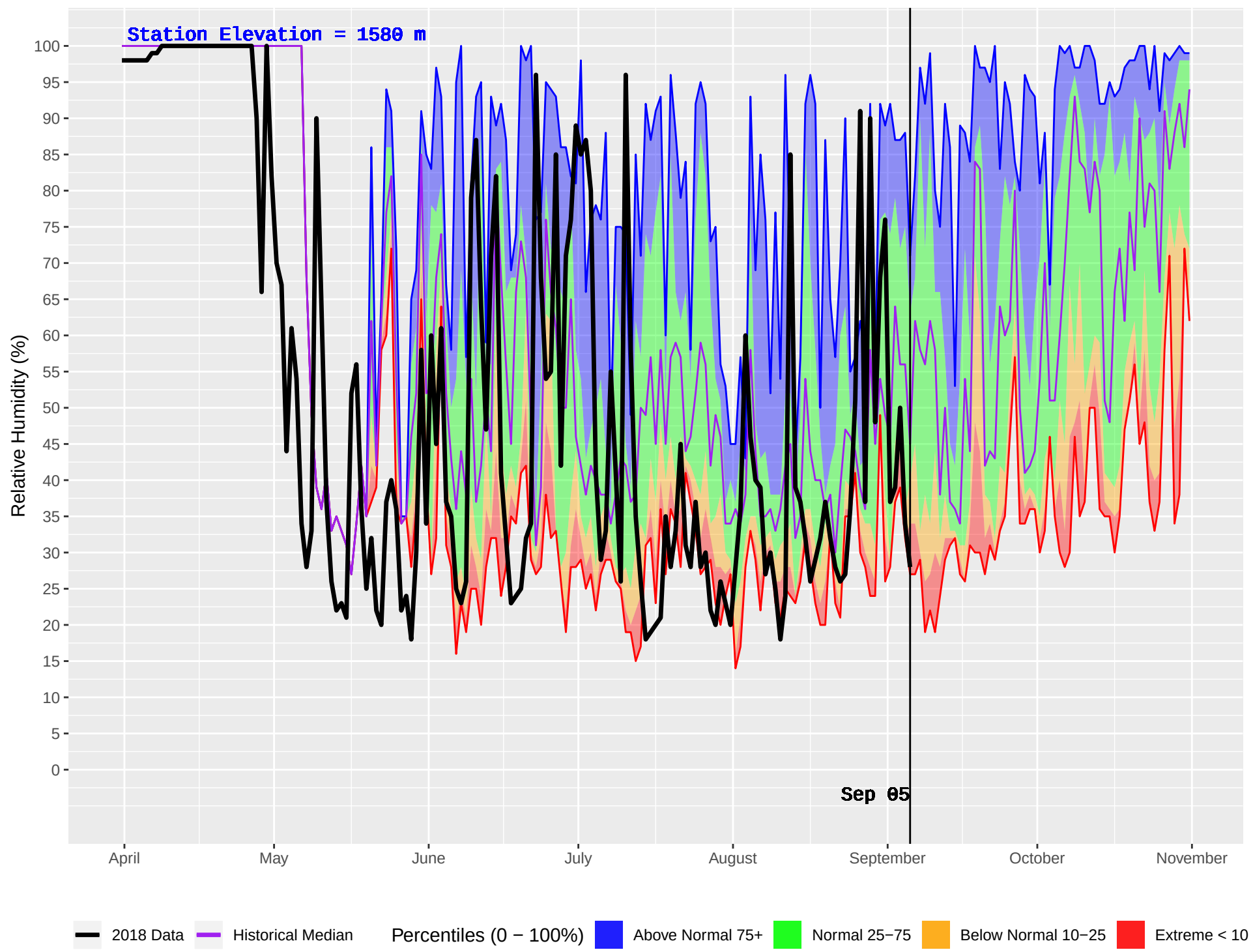
RORY CREEK (1092) : Historical (2010–2016) and Current (2018) Daily Relative Humidity
